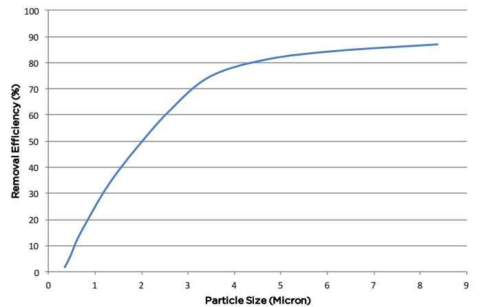
Particle Removal Efficiency
