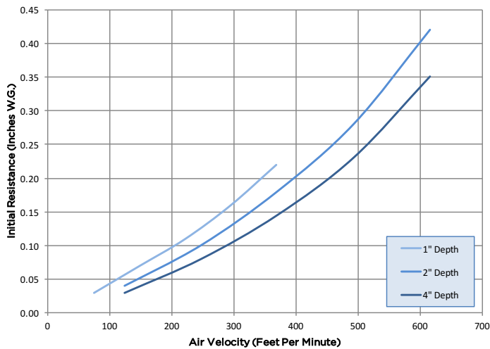
HD Pleat Initial Resistance
